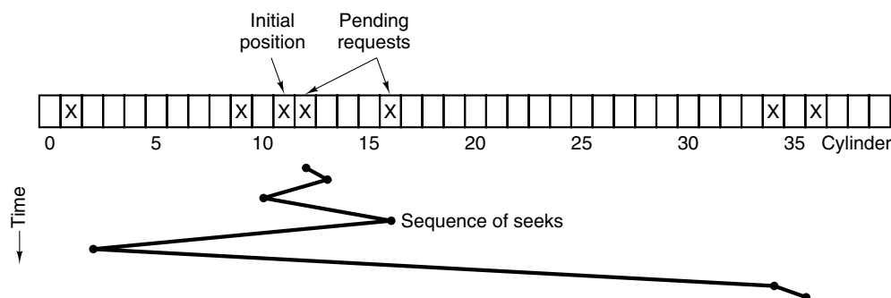
Figure 3-21. Shortest Seek First (SSF) disk scheduling algorithm.
