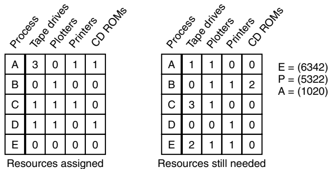
Figure 3-15. The banker's algorithm with multiple resources.
