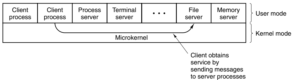
Figure 1-20. The client-server model.
