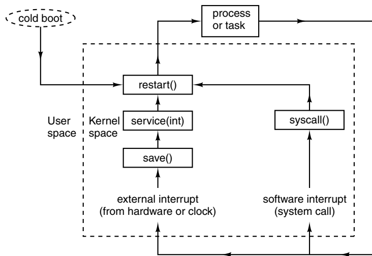
Figure 2-41. Restart is the common point reached after system startup, interrupts, or system calls. The most deserving process (which may be and often is a different process from the last one interrupted) runs next. Not shown in this diagram are interrupts that occur while the kernel itself is running.
