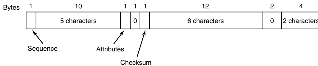
Figure 5-14. An entry for (part of) a long file name in Windows 98.
