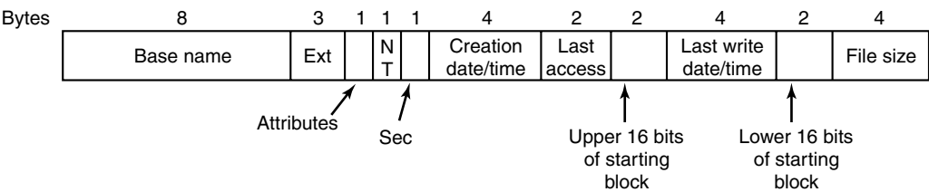
Figure 5-13. A Windows 98 base directory entry.
